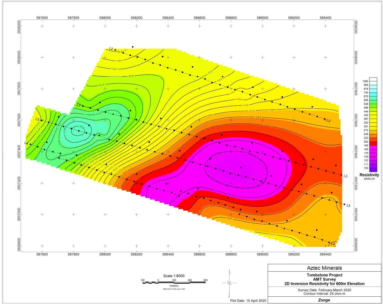
Figure 12. Contour map of 2D Inversion results for 600 m elevation.
