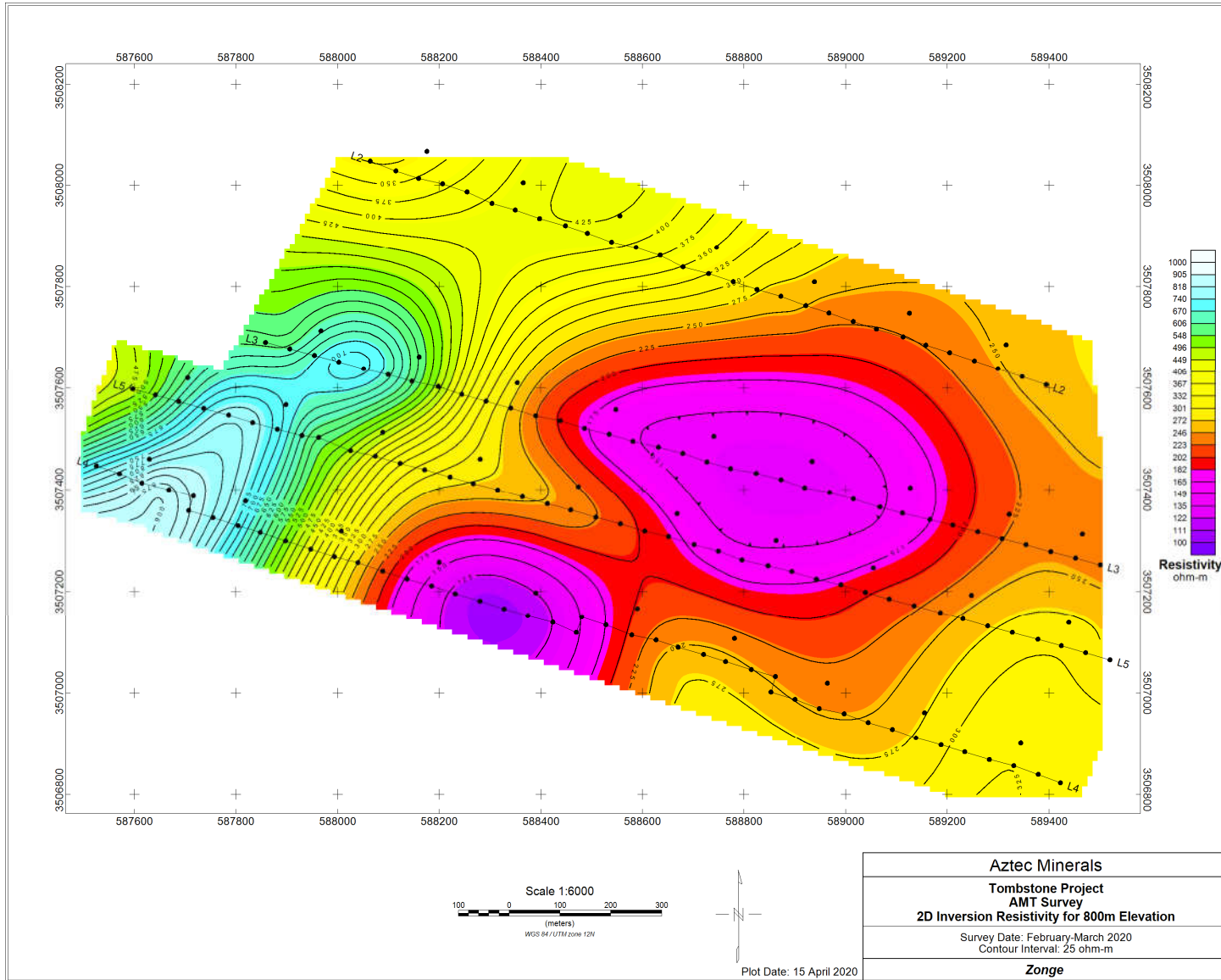
Figure 11: Contour map of 2D Inversion results for 800 m elevation.
