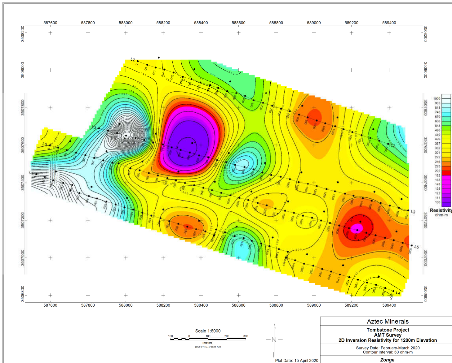
Figure 9: Contour map of 2D Inversion results for 1200 m elevation.
