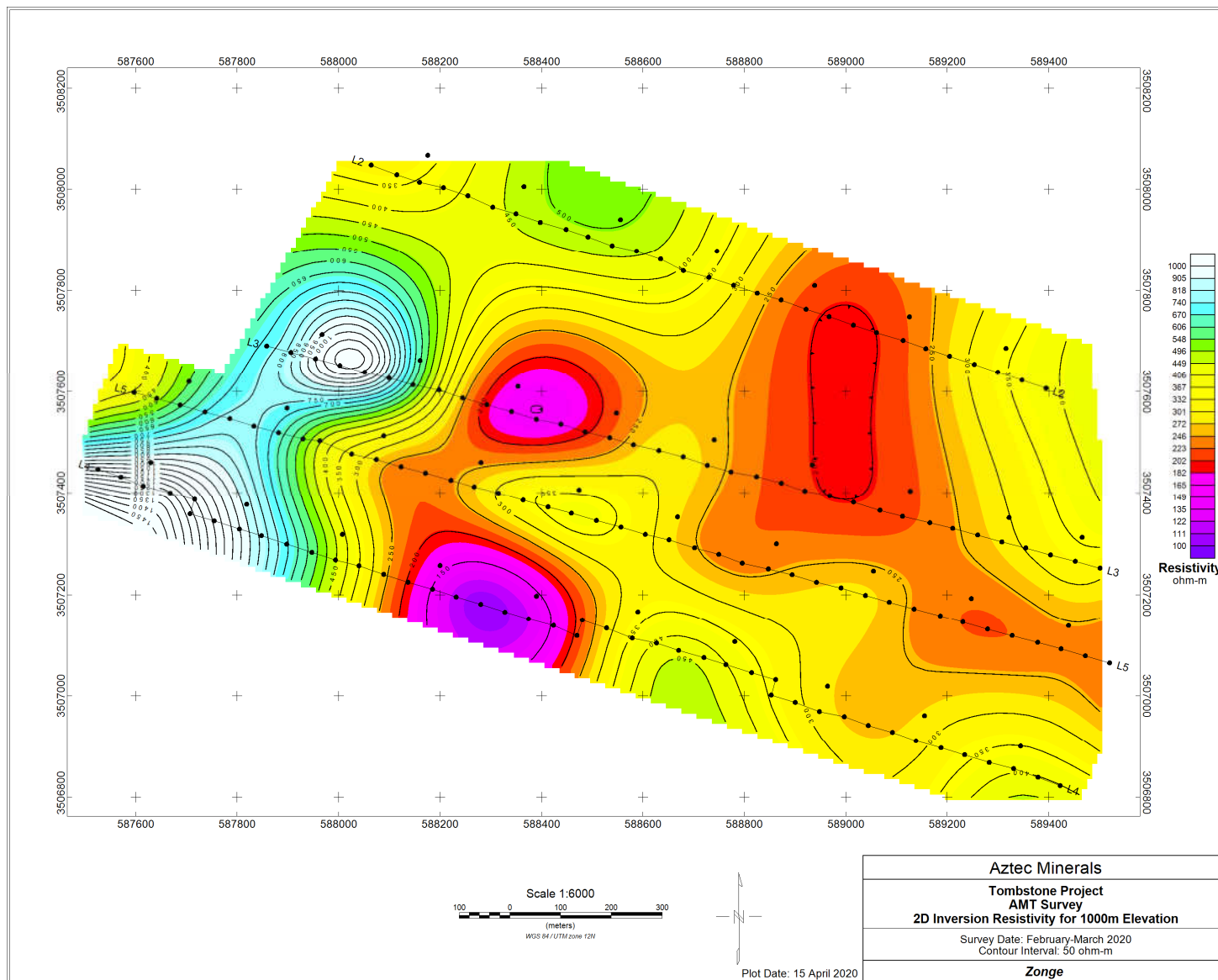
Figure 10. Contour map of 2D Inversion results for 1000 m elevation.
