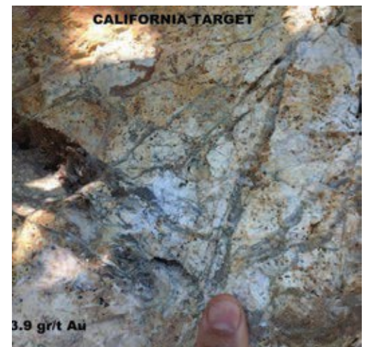
California zone mineralized stockworks in altered and brecciated high level porphyry intrusion grading 3.9 gpt gold in outcrop
